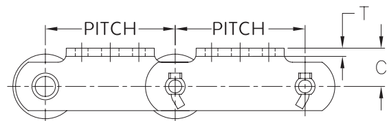
K1/K2 Attachment
