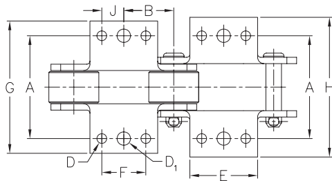
K1/K2 Attachment
