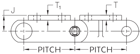
K2 Attachment
