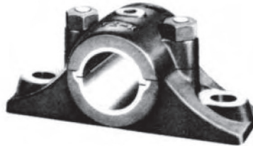
Type K Split Babbitted Bearing. Gibs are molded in the Babbitt lining. Supplied babbitted only with two cap bolts and two base mounting holes.
