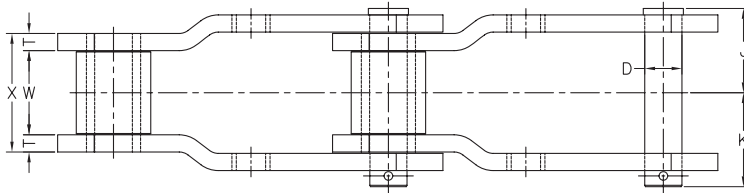
M14 Attachment
