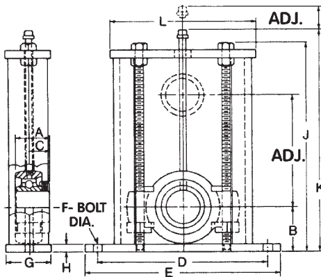
Type SG Ball Bearing
