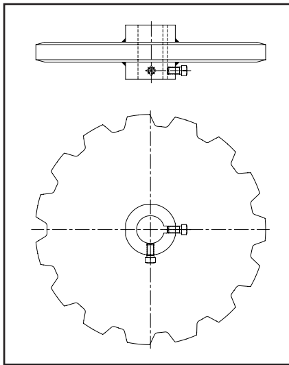
Standard Sprocket
